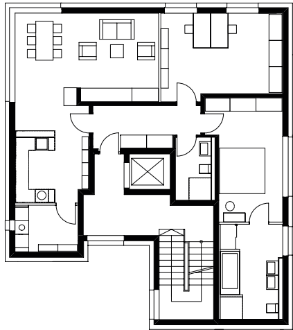
Grundriss Penthouse Penthouse floor plan
