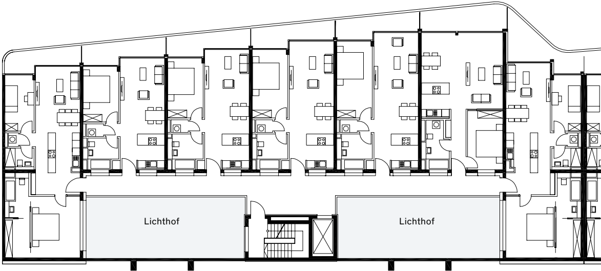
Ausschnitt Regelgeschoss Apartmenthaus Sector regular floor plan apartments
